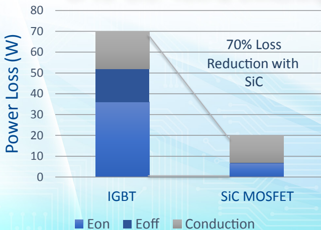
Si vs. SiC: 40kHz Switching
